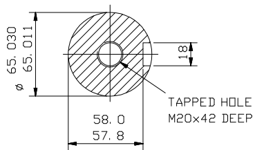
SECTION THROUGH SHAFT EXTENSION (SCALE 1: 2)
